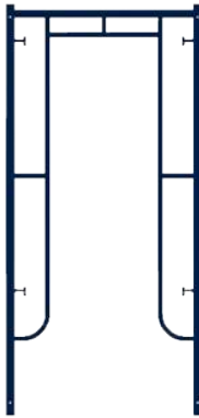
BFO3W67HH48 3'x6'7" Open End Frame 1.63" H-Lk 36.2 lbs.
