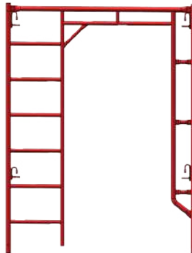
B-FOL5W67H-D48 5'x6'7" Open End Ladder Frame 1.625", D-Lk 48" Spacing 58.6 lbs.
