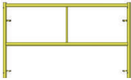
C-FS5W3H-Q24 5'x3' Step Frame 1.69", Q-Lk 24" Spacing 27.8 lbs.
