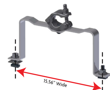
LDRSAUBG SAU Ladder Bracket (Channel Style) 5.8 lbs.
