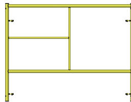
C-FS5W4H-Q36 5'x4' Step Frame 1.69", Q-Lk 24" Spacing 31.8 lbs.
